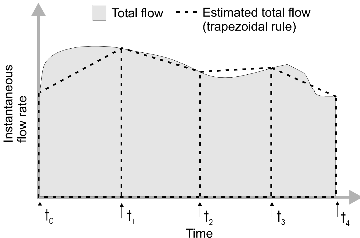
FIGURE 1 - Total Flow vs. Instantaneous Flow Rate
